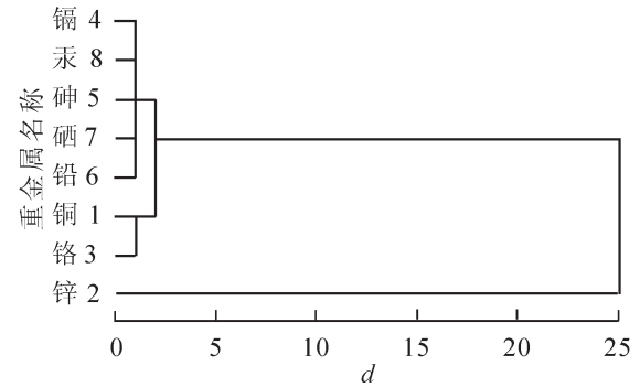
图2 高虹镇本地稻米R型聚类分析结果 Figure 2 R-cluster analysis of heavy metal concentrations for local rice samples in Gaohong Town
