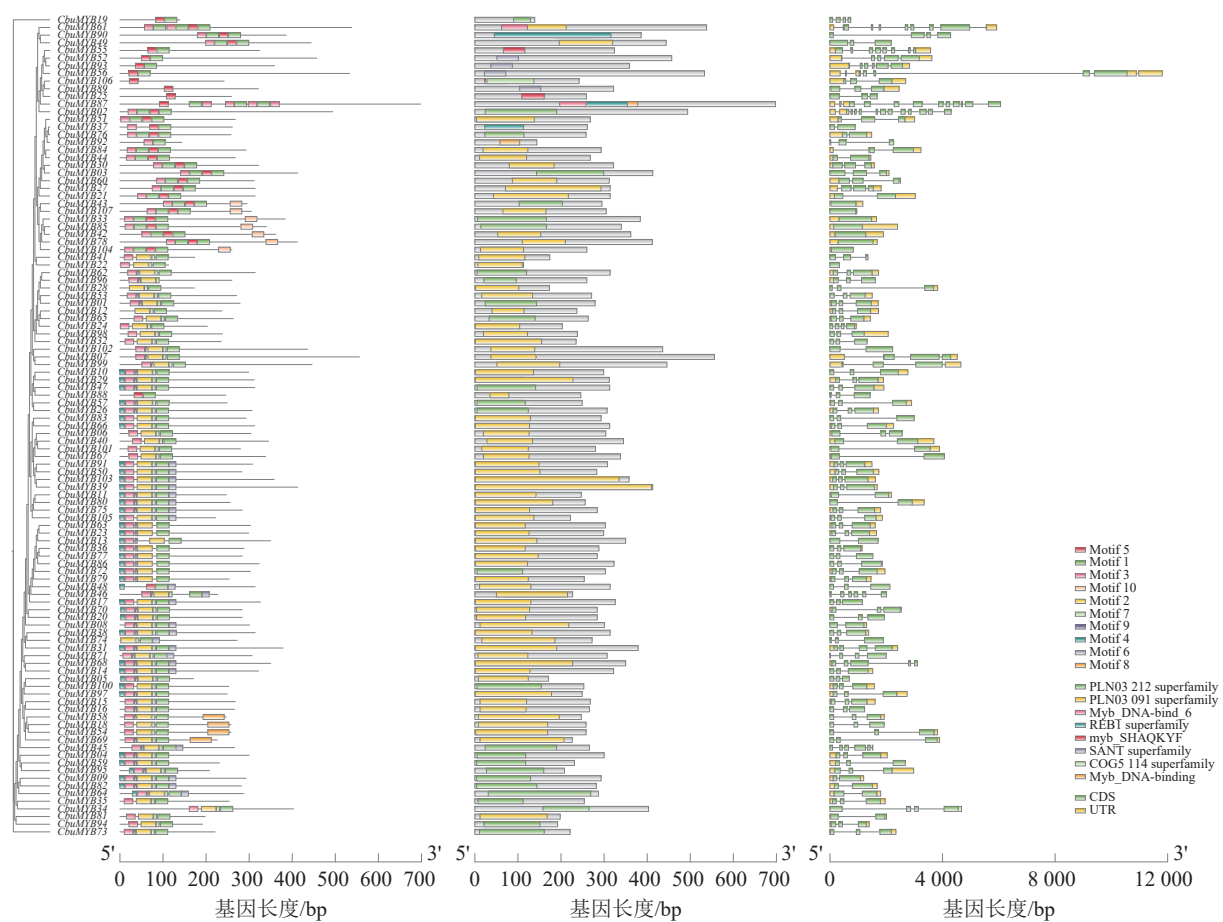
附图 1 CbuMYB 基因家族基序、保守结构域及基因结构 Supplementary figure 1 Motifs, conserved domains and gene structures of the CbuMYB gene family
