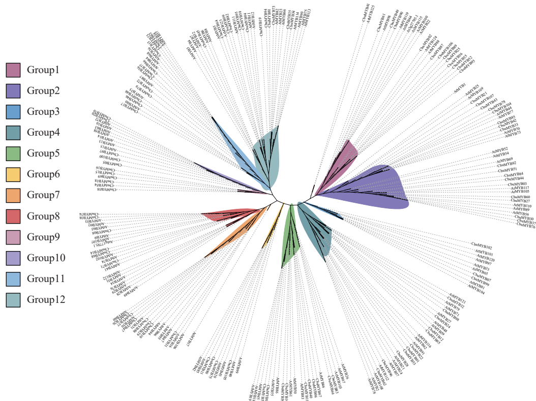
附图2 CbuMYB 与 AtMYB 基因家族进化关系分析 Supplementary figure 2 Evolutionary relationship between CbuMYB and AtMYB
