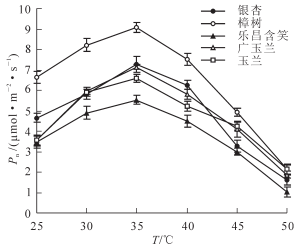
图 3 5 个树种叶片光合速率对温度的响应曲线 Figure 3 Response of photosynthetic rate to temperatures of five species
