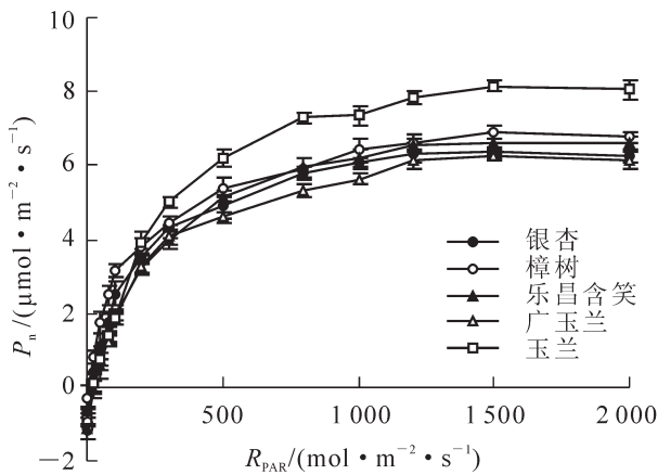
图 2 5 个树种叶片光合速率对光强的响应曲线 Figure 2 Response of photosynthetic rate to light intensity of five species
