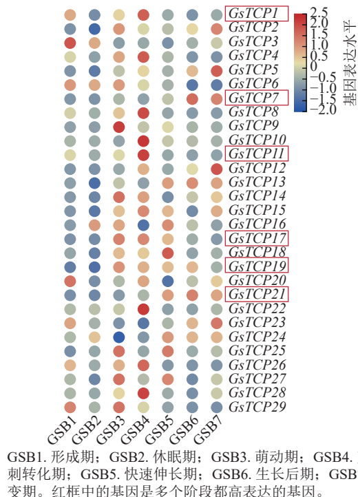
图 5 GsTCP 在皂荚刺不同发育阶段的表达模式分析 Figure 5 Expression patterns of GsTCP at different developmental stages of G. sinensis thorns
