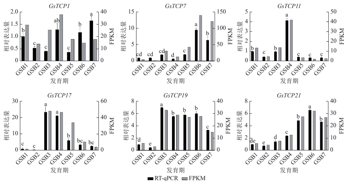
图 6 RT-qPCR 验证 GsTCP 家族基因在不同发育期皂荚刺中的表达 Figure 6 RT-qPCR validation of GsTCP gene family expression in G. sinensis thorns at different developmental stages
