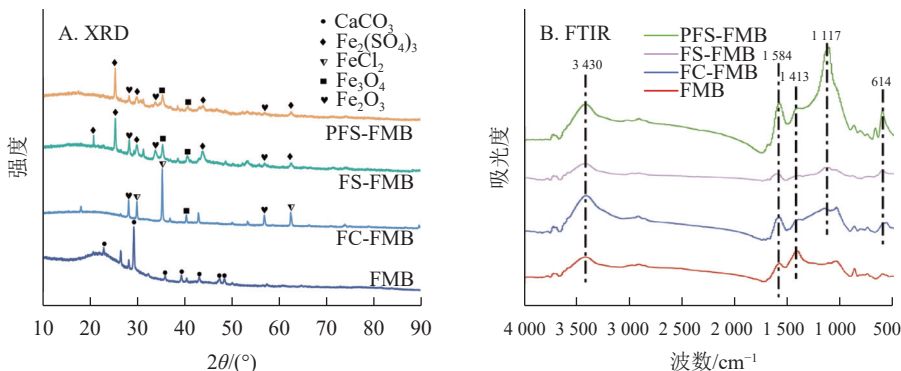
图 2 生物质炭的 X 射线衍射分析 (XRD) 图谱和傅里叶红外光谱 (FTIR) 图 Figure 2 X-ray diffraction analysis (XRD) pattern and Fourier Transform Infrared Spectroscopy (FTIR) pattern of biochars
