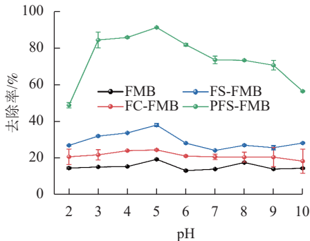
图 4 pH 对不同生物质炭去除 As(Ⅲ) 的影响 Figure 4 Effect of pH on the removal of As(Ⅲ) by different biochars
