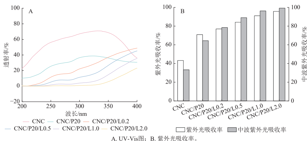
图 6 CNC 和 CNC/PCNF/LNPs 薄膜的 UV-Vis 图和紫外光区及中波紫外光区的紫外光吸收率 Figure 6 UV-Vis images, UV absorption in the UV region and the UVB region of CNC and CNC/PCNF/LNPs films
